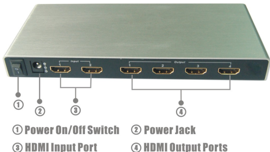
Figure 2. Rear Panel Layout
